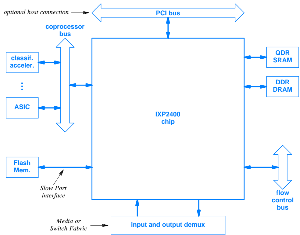
Figure 15.9 Illustration of external connections supported by Intel's IXP2400 network processor.
