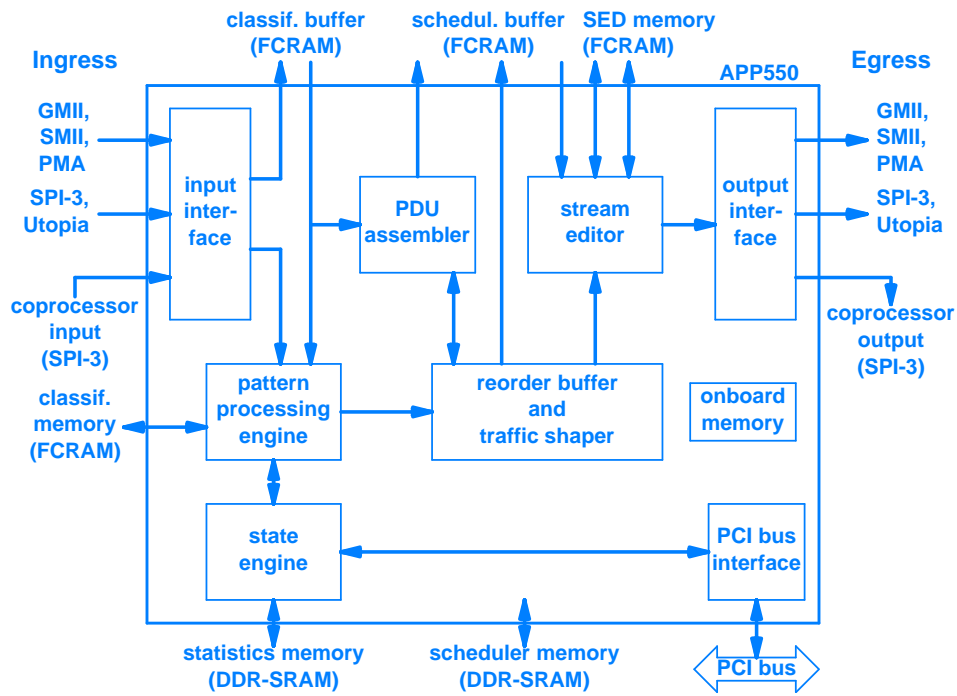
Figure 17.10 Conceptual organization of Agere's APP550 showing the logical connections among major components on the chip and external components. The chip contains additional connections that are not shown.
