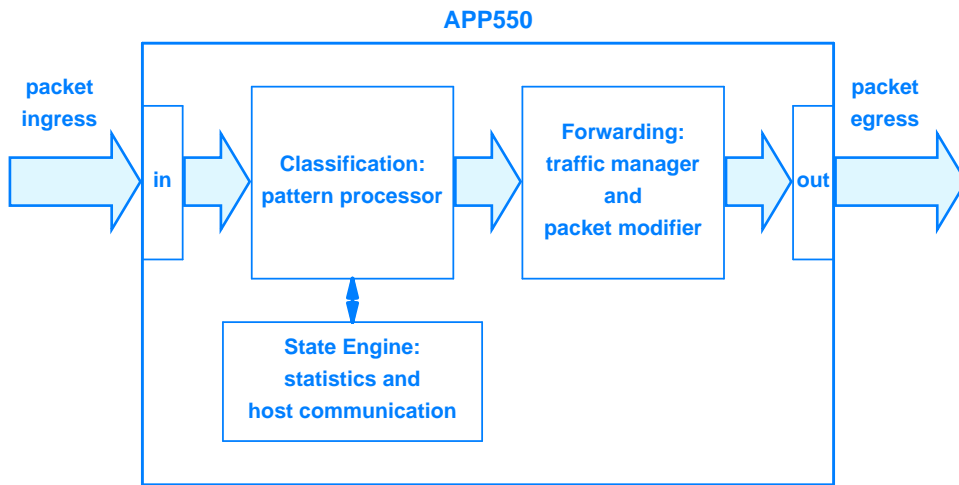
Figure 17.4 Second generation implementation of Agere's PayloadPlus network processor architecture. A single APP550 chip contains three function blocks plus I/O interface mechanisms.
