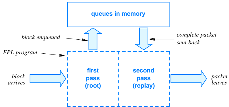
Figure 20.1 Illustration of the conceptual flow of data through an FPL program. The first pass is invoked once for each block; the second pass is invoked once for a packet.
