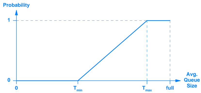
Figure 22.3 A plot of Equation 22.1 that shows linear behavior. The probability must be computed without using multiplication or division.
