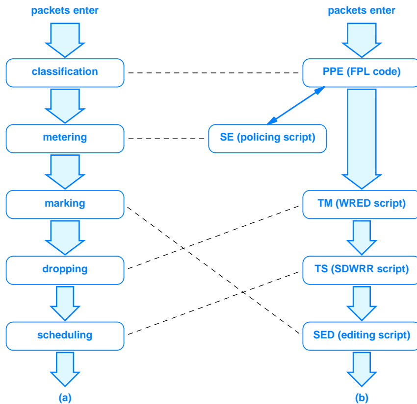
Figure 24.4 (a) The DiffServ conceptual processing model, and (b) the implementation on an APP550, with smaller arrows indicating possible reduced flow resulting from dropped packets. Dashed lines show how the implementation corresponds to the model.
