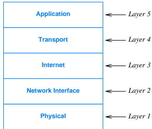
Figure 3.1 The Internet 5-layer reference model. Layer 2 is also known as the link layer , data link layer , or MAC layer .
