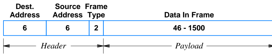
Figure 3.2 The Ethernet frame format as seen by a network system. Numbers give the size of each field measured in 8-bit octets.
