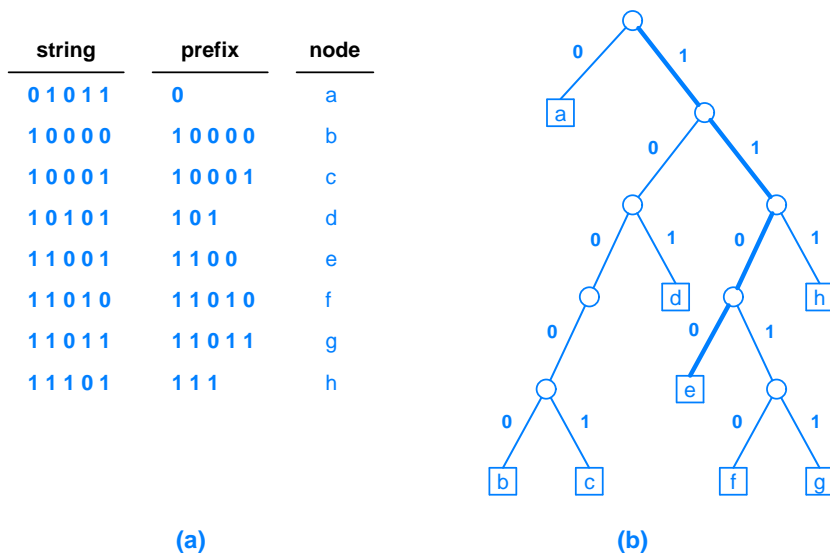
Figure 5.7 (a) A table of binary strings, their unique prefixes, and a node in the trie, and (b) a binary trie for the prefixes with the path corresponding to 1100 (e) darkened. Strings used in an IP routing table are 32 bits long.
