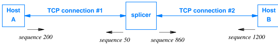
Figure 5.8 Illustration of TCP splicing. Labels show the initial sequence numbers that each side of a connection have chosen for outgoing data.
