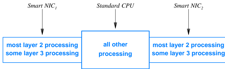
Figure 8.5 Hardware architecture of an optimized system with smart network interface cards. Because each NIC performs more processing, the CPU load is reduced.
