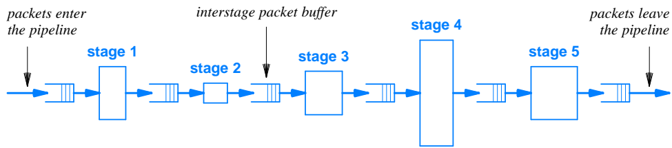
Figure 8.6 Illustration of a 5-stage data pipeline. The size and complexity of hardware varies among stages because the processing performed by a given stage differs from the processing performed by other stages.
