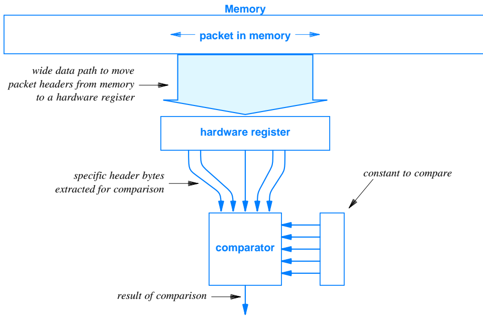
Figure 9.2 A hardware architecture for optimized classification. Packet headers are moved to a register; selected octets are extracted and compared to a constant value.
