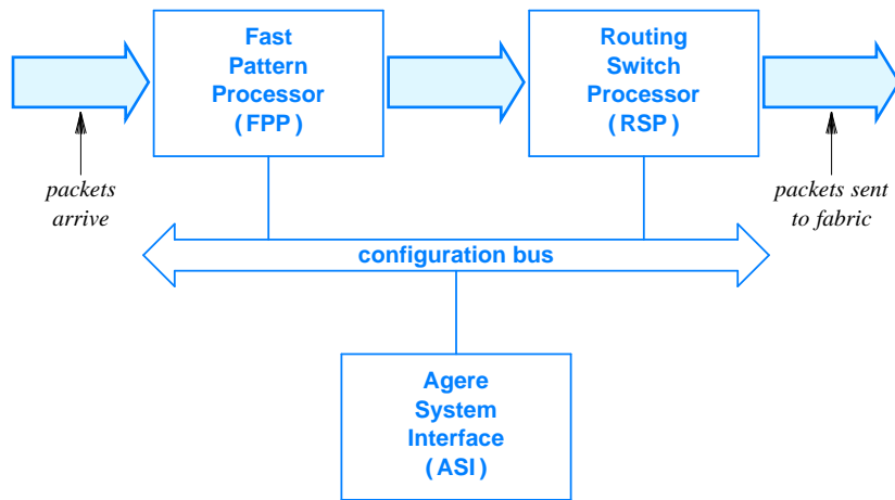
Figure 15.1 Illustration of Agere's network processor architecture; three separate chips are interconnected to form a pipeline.
