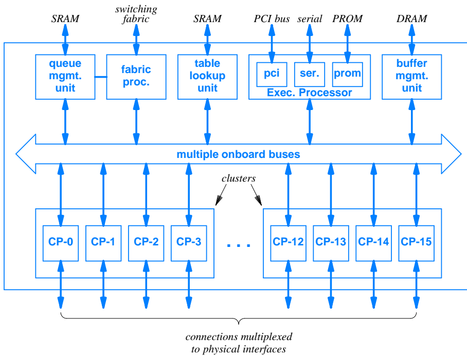
Figure 15.16 The internal architecture of Motorola's C-Port chip. The diagram shows the sixteen channel processors (labeled CP-0 through CP-15) configured in parallel clusters of four channel processors per cluster.
