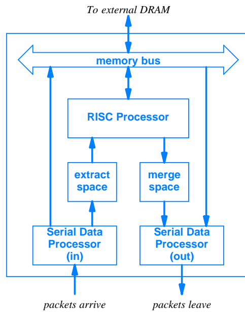
Figure 15.17 The internal architecture of a single CP with a RISC core plus functional units to handle ingress and egress. Each C-Port chip contains a total of sixteen CPs.
