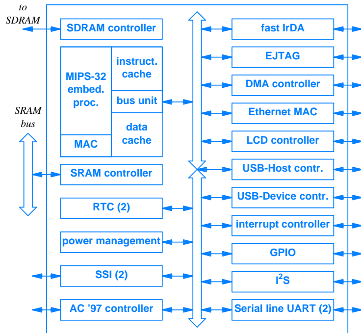
Figure 15.6 The internal architecture of Alchemy's Au1000 chip. Two internal buses provide interconnections: a system bus (the top bus) and a peripheral bus (the bottom bus).
