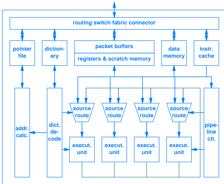
Figure 15.9 The internal structure of a Cognigine network processor (RCU). The pipeline controller can reconfigure data paths.
