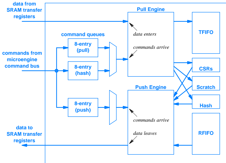
Figure 20.10 A simplified illustration of the FBI architecture on Intel's IXP1200. The Push Engine and Pull Engine operate in parallel.
