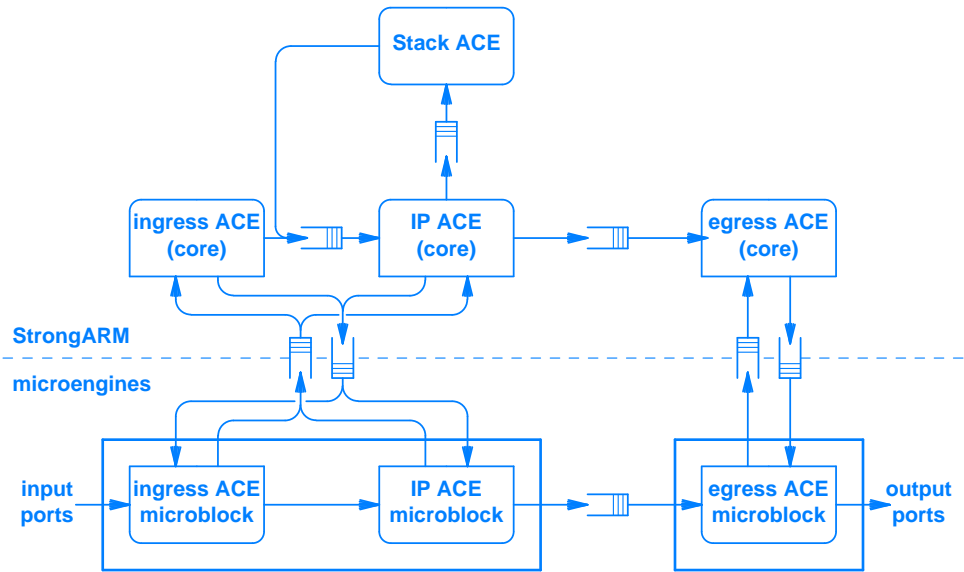
Figure 22.6 Illustration of communication queues used with ACEs. Queues permit processors to execute in parallel.
