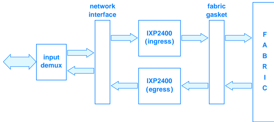
Figure 27.1 Illustration of the packet flow through two IXP2400 chips configured to handle data rates of OC-48 or higher. One chip handles ingress processing and the other handles egress.
