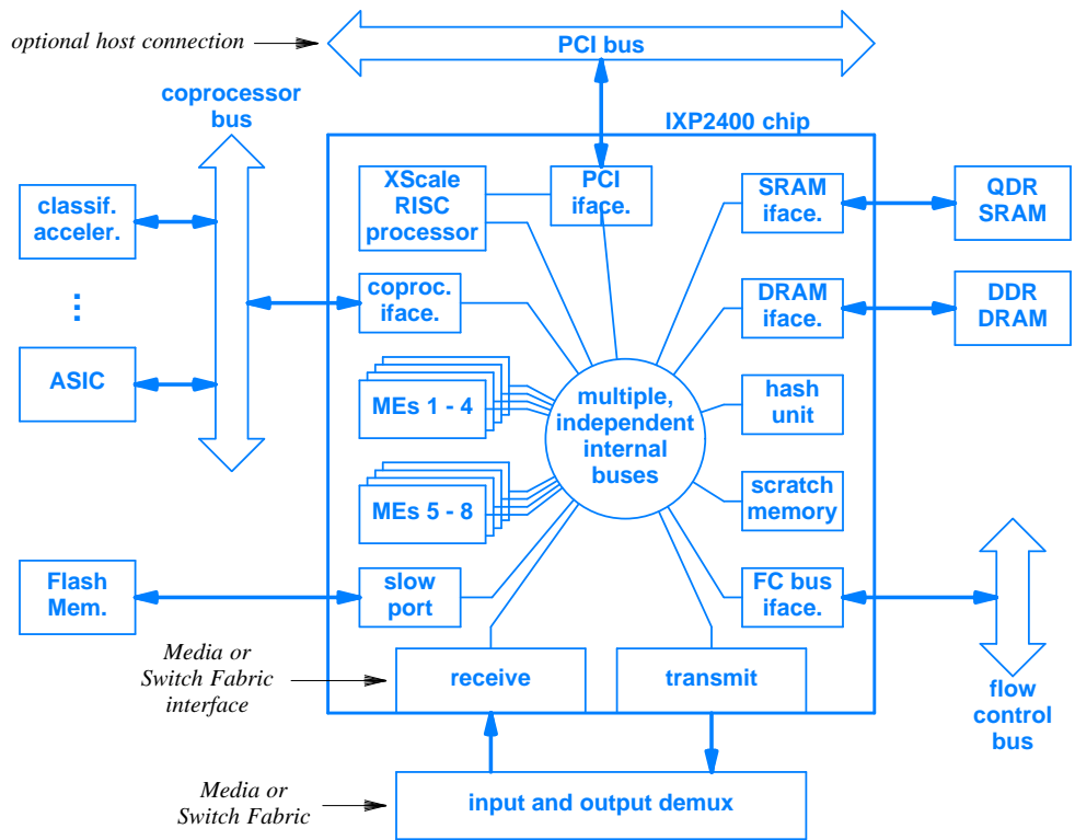
Figure 27.3 Illustration of the internal architecture of an Intel IXP2400. The chip contains additional functional units not shown.
