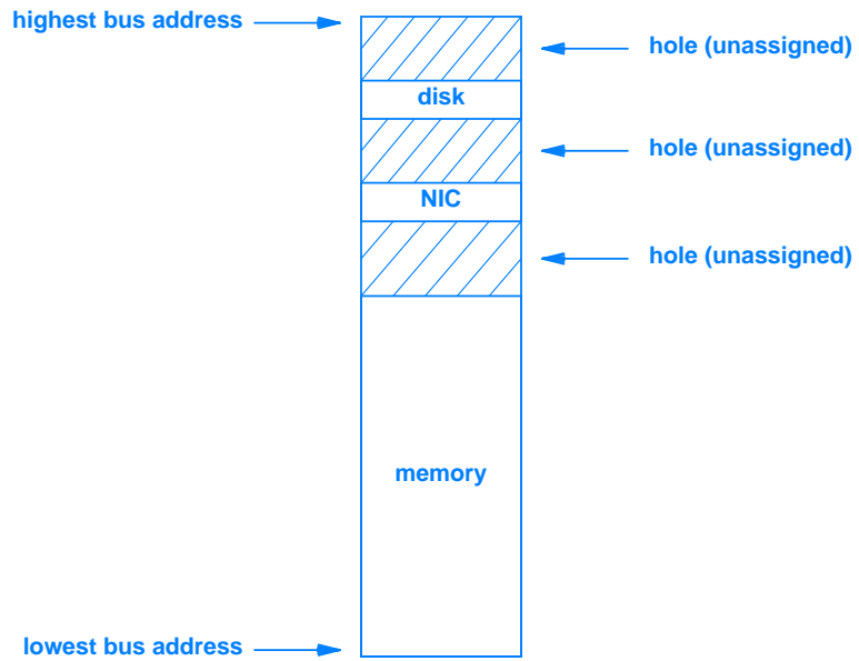
Figure 4.3 An example bus address space occupied by a disk device, a network interface device, and memory. Holes occur when no hardware device has been assigned to an address.
