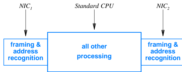
Figure 8.1 The hardware architecture used with a software-based network system. The CPU handles all protocol processing tasks except for framing and onboard address recognition.
