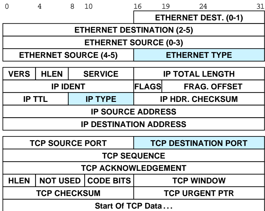
Figure 9.1 Illustration of encapsulated headers at the beginning of a packet shown with extra space between Ethernet, IP, and TCP headers. Highlighted fields are used to determine if the packet is destined for a web server.
