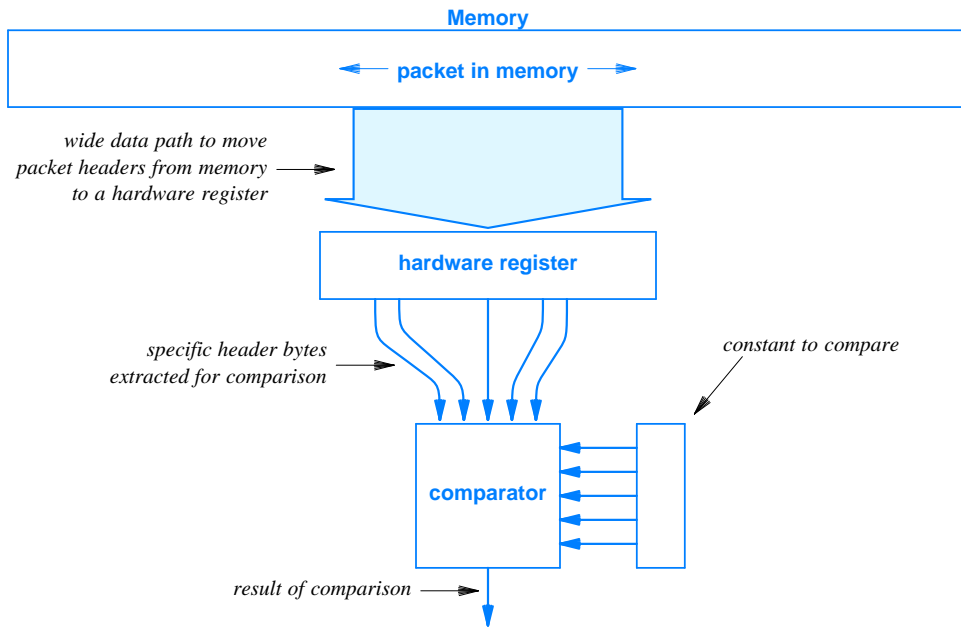
Figure 9.2 A hardware architecture for optimized classification. Packet headers are moved to a register; selected octets are extracted and compared to a constant value.
